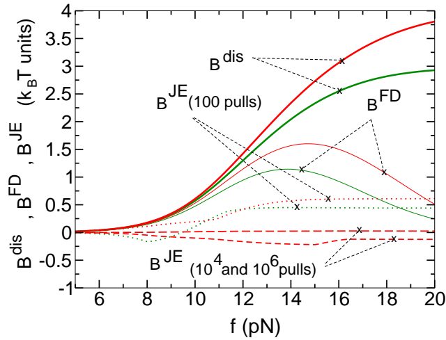
Figure 12: Behavior of the different bias defined in (25,26,27) along the force coordinate. Figure taken from [23].
