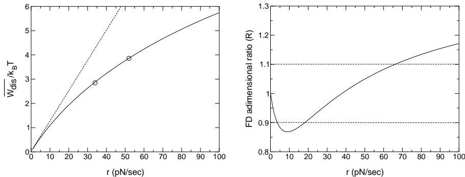
Figure 10: Average dissipated work (left) and fluctuation-dissipation ratio R (right) as a function of the pulling speed. The circles in the left figure are the experimental values. The values of the kinetic parameters characterizing the rates (22) have been chosen to fit the experimental data. The dashed line in the left figure shows the linear-response formula (24). The two horizontal dashed lines in the right figure limit a region of pulling speeds where the FD estimate (21) is expected to approximate well the free-energy change during the folding-unfolding reaction. Figure taken from [23].
