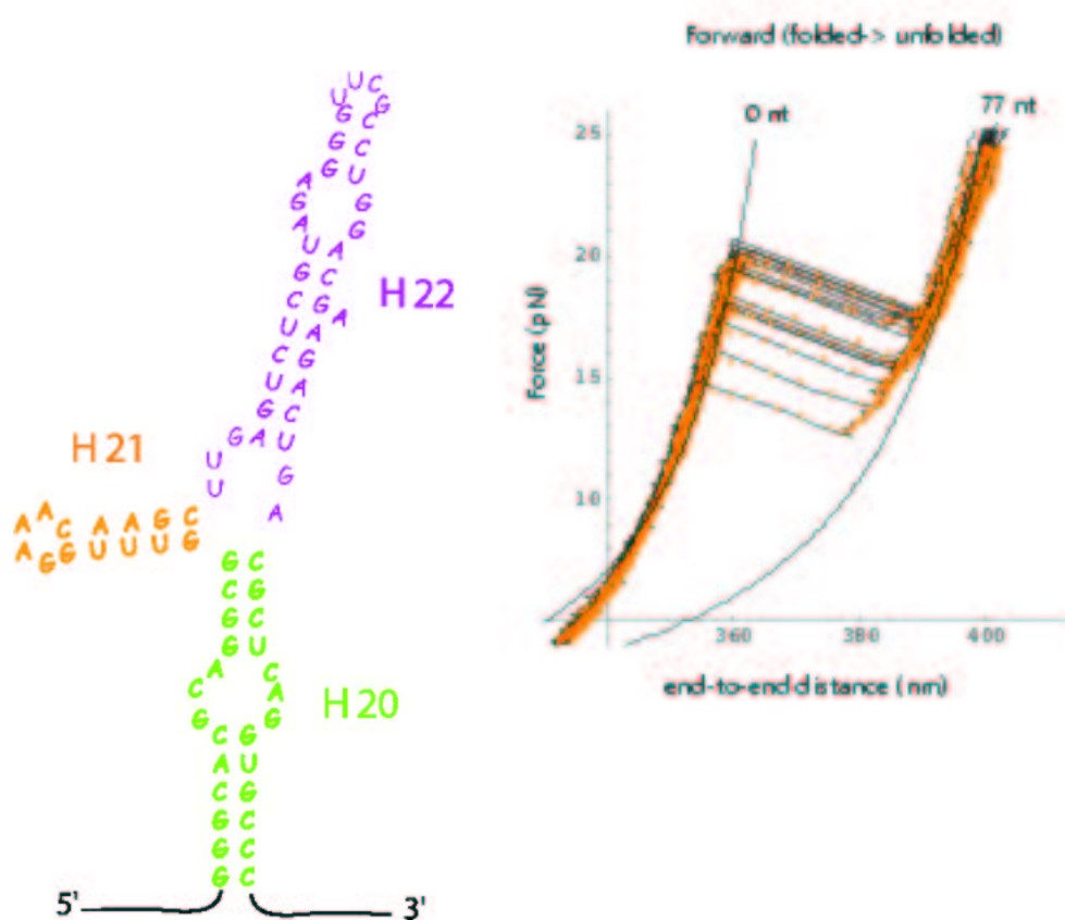
Figure 8: The left figure shows the structure of the junction in the 16S domain of the 30S ribosomal RNA subunit. The right figure shows some unfolding curves at 3.5pN/s. Courtesy of Delphine Collin.
