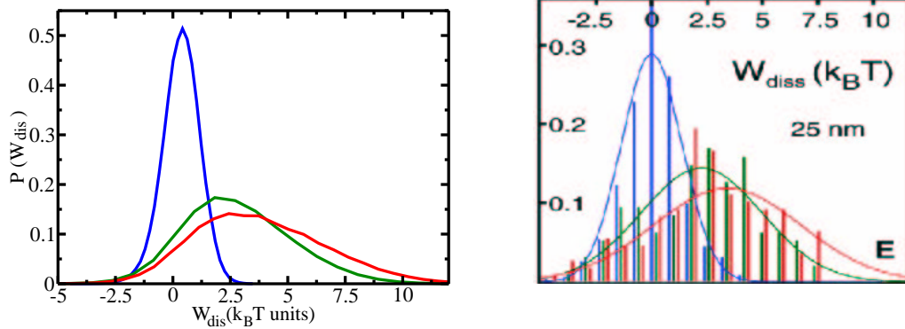
Figure 11: Work distributions obtained for the model (left) compared to the experimental results. Strong deviations from a Gaussian behavior are predicted, specially in the left tails of the distribution. Figures taken from [23, 81].
