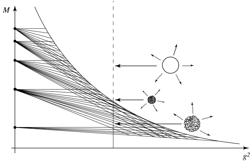
Figure 4: Evolution of the energy levels of massive string states as the string coupling g increases. String states are expected to transform into black-hole states on the correspondence line g^2 M \sim M_s . Vertical line: Corresponding transformation of a black hole, losing mass at fixed g under Hawking radiation, into an initially compact string state, which inflates before decaying into massless radiation.
