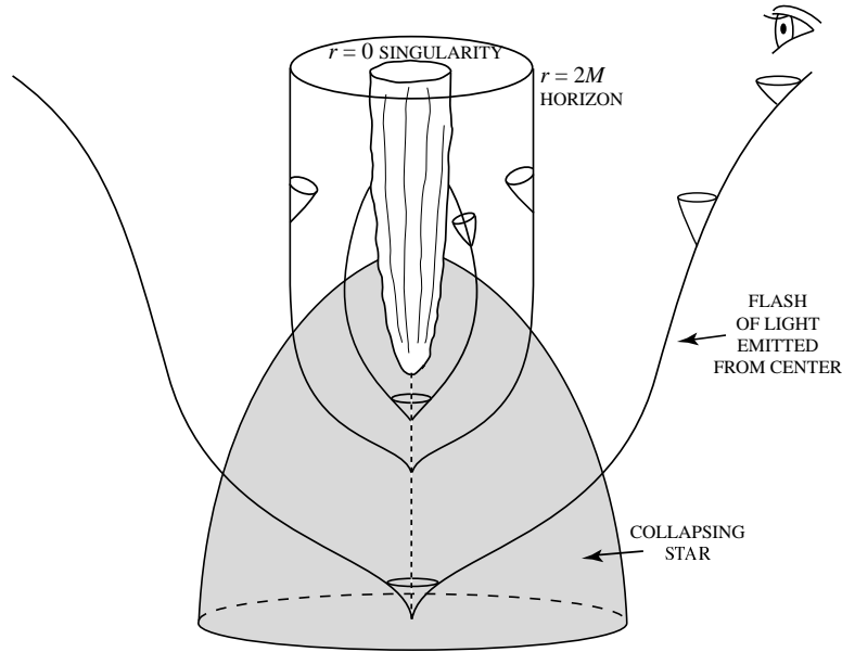
Figure 1: Spacetime representation of the formation of a black hole by the collapse of a star. The horizon is the spacetime history of a bubble of light ( i.e. a null hypersurface) which stabilizes itself under the strong pull of relativistic gravity
