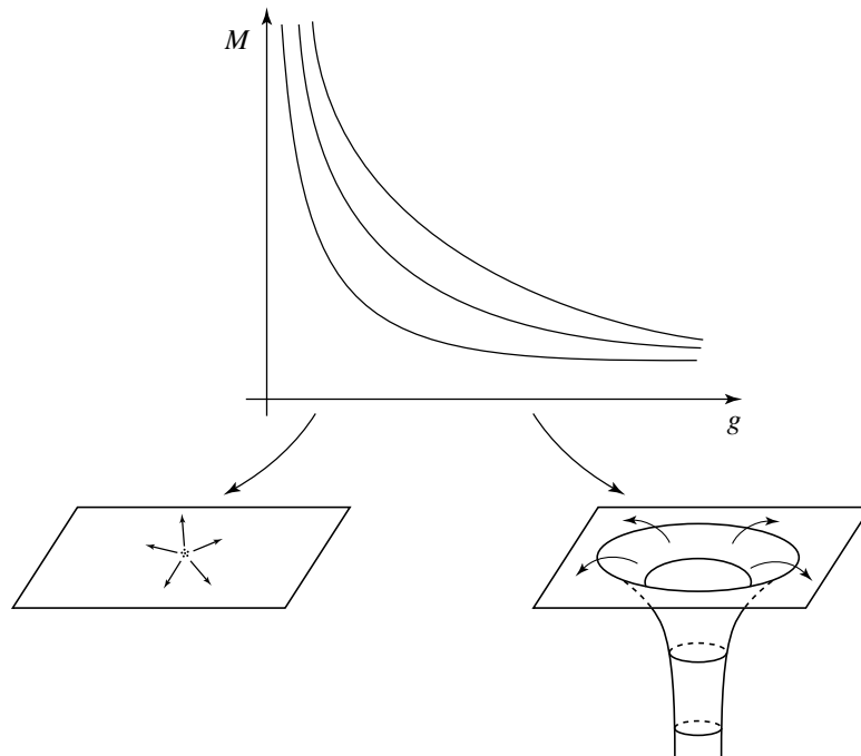
Figure 3: Evolution of the mass-energy, and of the physical structure, of an initially point-like configuration of D -branes as the string coupling g increases.
