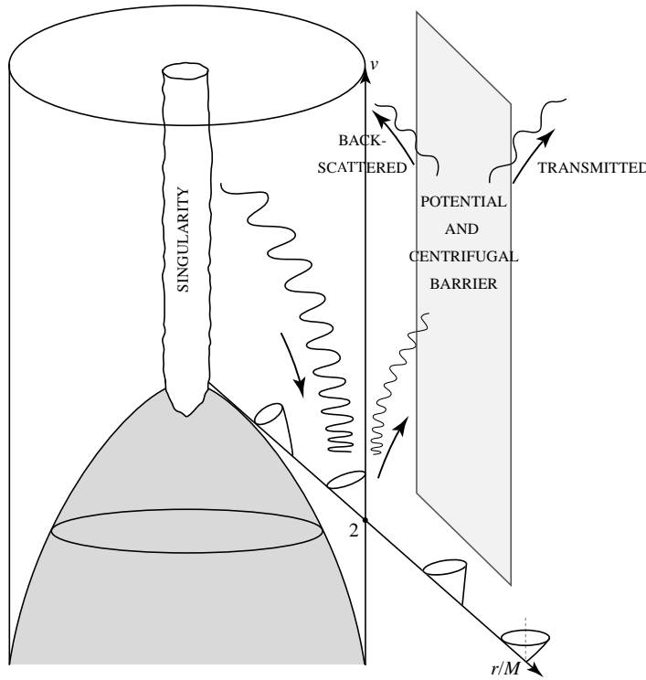
Figure 2: Splitting of an initial negative-frequency mode straddling the horizon into a mode falling into the black hole, and an outgoing mode which, after being partially reflected back into the black hole by the potential barrier representing gravitational and centrifugal effects, ends up as positive-frequency Hawking radiation at infinity. The antiparticle mode falling into the black hole can be interpreted as a particle traveling backwards in time, from the singularity down to the horizon [25] (hence the downwards orientation of the arrow).
